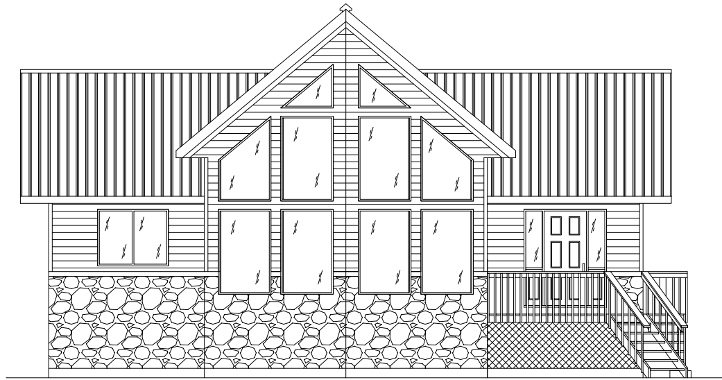
FRONT ELEVATION
